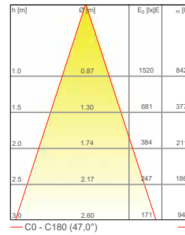
46°- P05 - 13,4W
