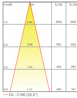
21°- P05 - 13,4W
