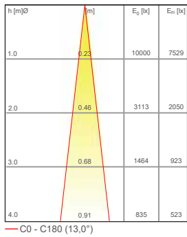
12°- P05 - 13,4W
