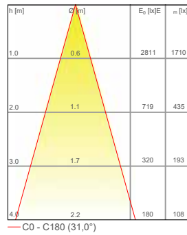
31°- P05 - 13,4W
