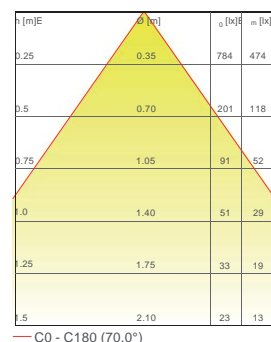
— C0 - C180 (70,0°)
