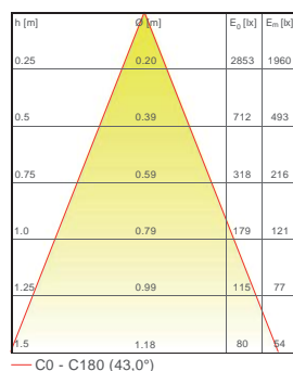
— C0 - C180 (43,0°)
