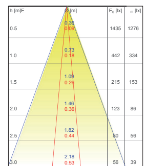
10°x40° - 2 Watt
