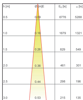
10° - 2 Watt
