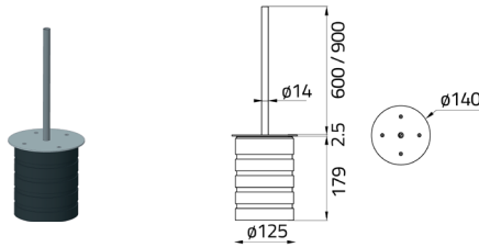
Base with housing box for power supply
