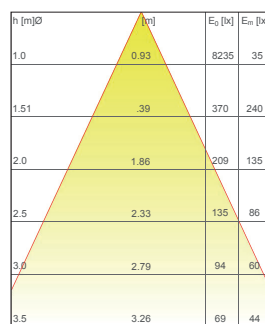
— C0 - C180 (50,0°)
